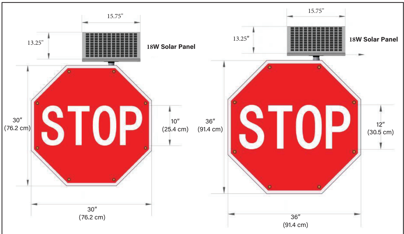
30" Solar LED Flashing Stop Sign ALC-SS-30 Sign Dimensions 30" x 30" Octagon, .160" thick, Weight: 25 lbs.
